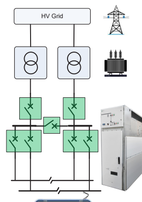
Typical AC traction substation
