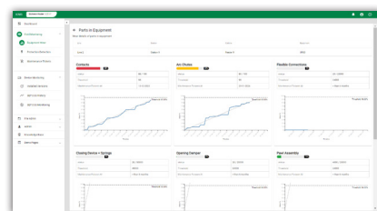
Wear details of parts in equipment
